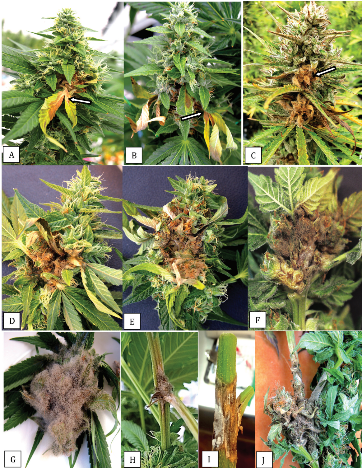
Fig. 1 (Colour online) Development of bud rot, caused by Botrytis cinerea , on cannabis inflorescences. a , Early symptom of an infected bract leaf turning yellow (arrow). b , Spread of the pathogen to several bract leaves (arrow). c , Necrotic areas on the inflorescences (arrow) due to pathogen spread. d , e , Internal decay due to pathogen development internally within the inflorescence. f , g , Sporulation of B. cinerea on infected tissues showing the characteristic grey mould symptom. h–j , Stem cankers developing at different locations on the plant.
